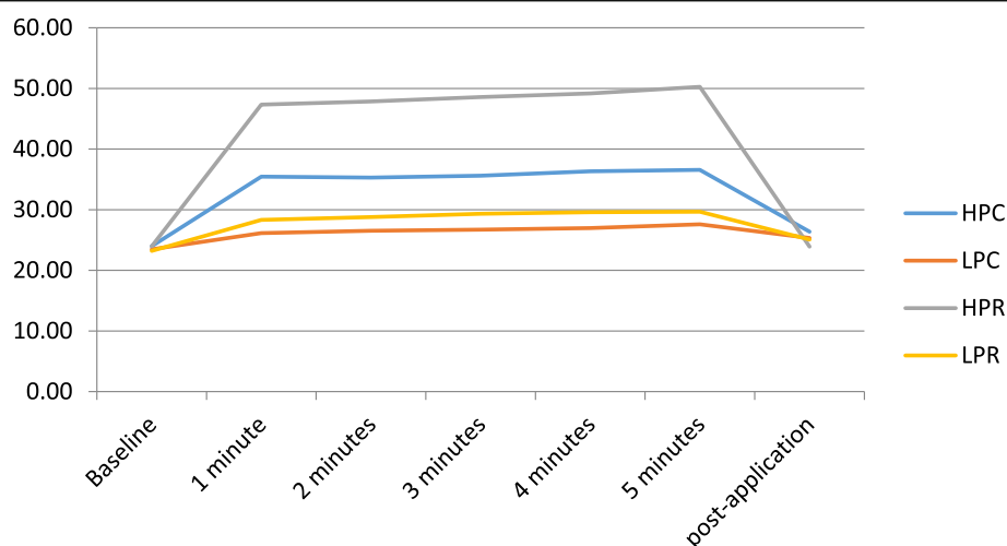
Fig. 4 Achilles tendon temperature. HPC: high-power capacitive; LPC: low-power capacitive; HPR: high-power resistive; LPR: low-power resistive
