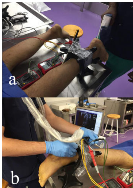
Fig. 2 a Temperature measurement with digital thermometer; b Thermocouple placement under ultrasound guidance; c Thermocouple position
