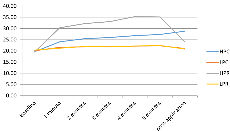
Fig. 5 Musculotendinous junction temperature. HPC: high-power capacitive; LPC: low-power capacitive; HPR: high-power resistive; LPR: low-power resistive
